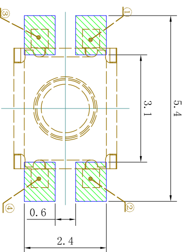
P.C.B MOUNTING PATTERN DIMENSION
